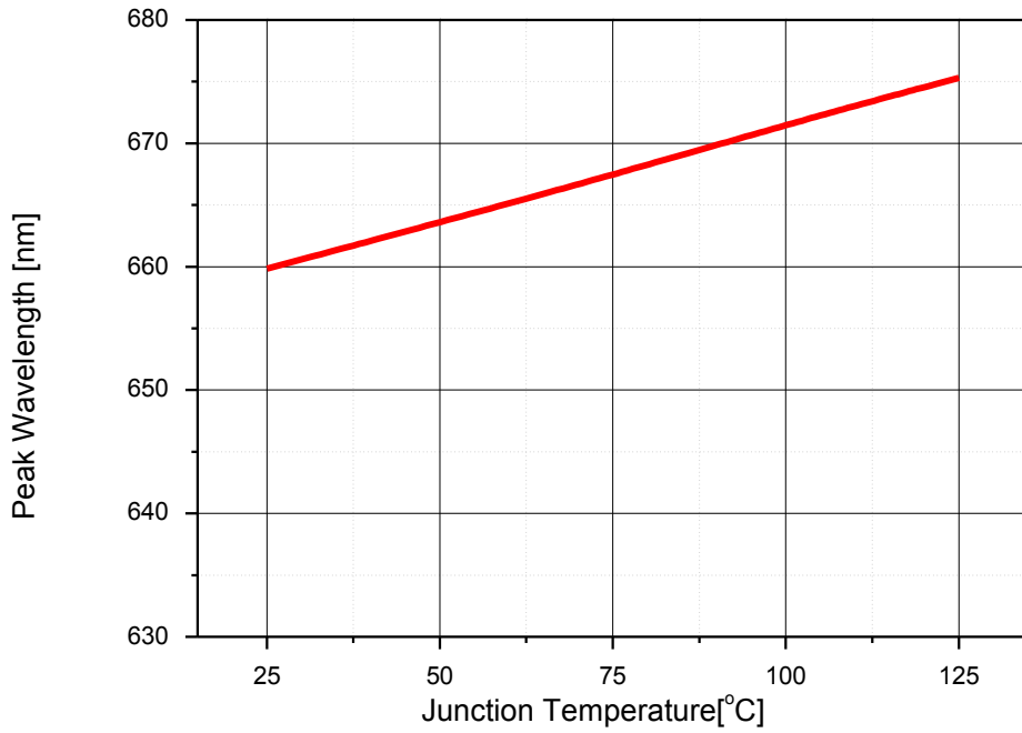
Junction Temperature vs. Peak Wavelength at IF=350mA
